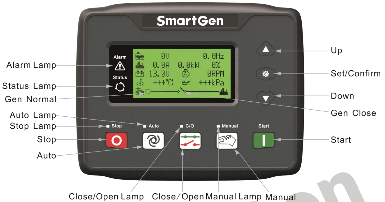
Fig. 1 HGM410N Front Panel
